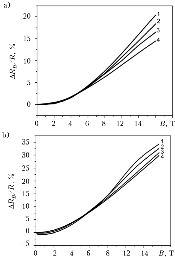
Fig. 3. The dependences of relative change of the resistance vs the magnetic field induction for the n - (a) and p -type conductivity of (b) Ge whiskers at different temperature:
