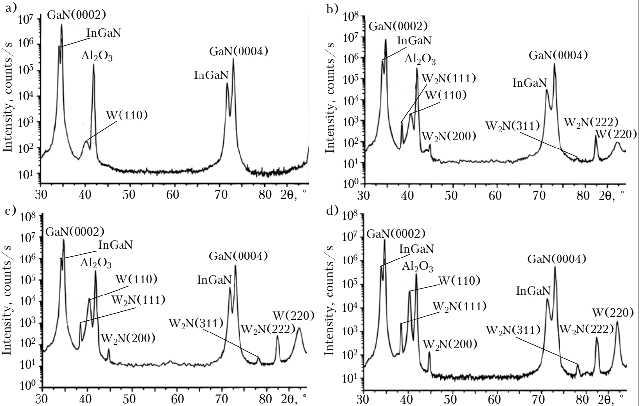
Рис. 3. XRD data for the W/ \text{InGaN} samples as-deposited (a) and annealed at 500°C (b), 700°C (c), and 950°C (d) [34]
